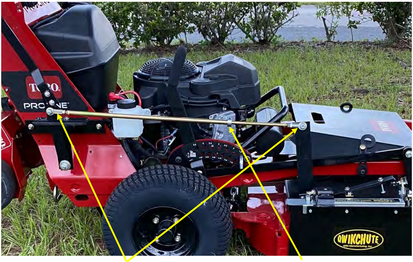
ROD ENDS
