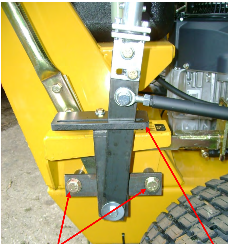
NEW 1/2" BOLTS
