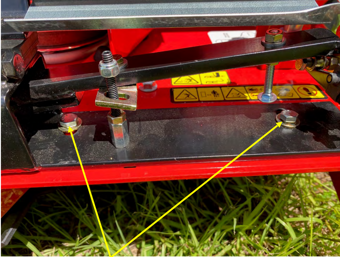
MOUNTING BOLTS AND LOCATION TO BE DRILLED
